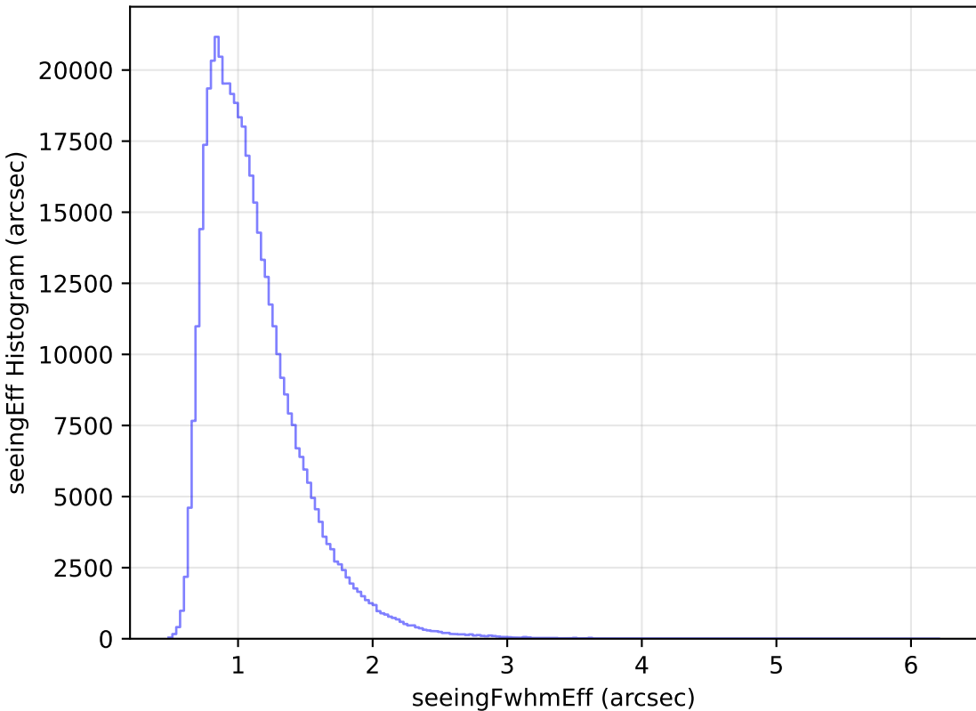
too_elab_heavy_r32_d2_ugrizy_v3.4_10yrs WFD r band: seeingEff Histogram
