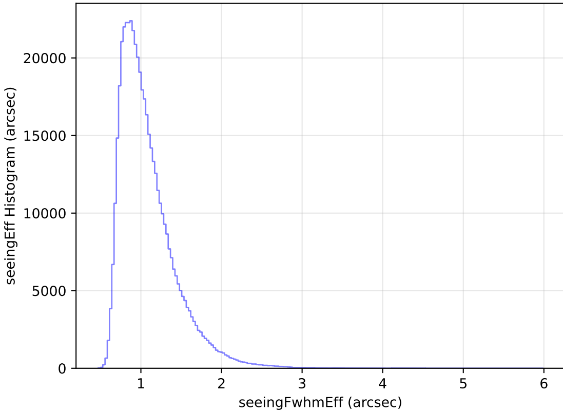
too_elab_heavy_r32_d2_ugrizy_v3.4_10yrs WFD i band: seeingEff Histogram
