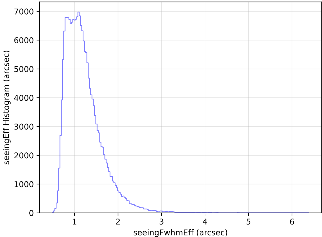
too_elab_heavy_r32_d2_ugrizy_v3.4_10yrs WFD g band: seeingEff Histogram
