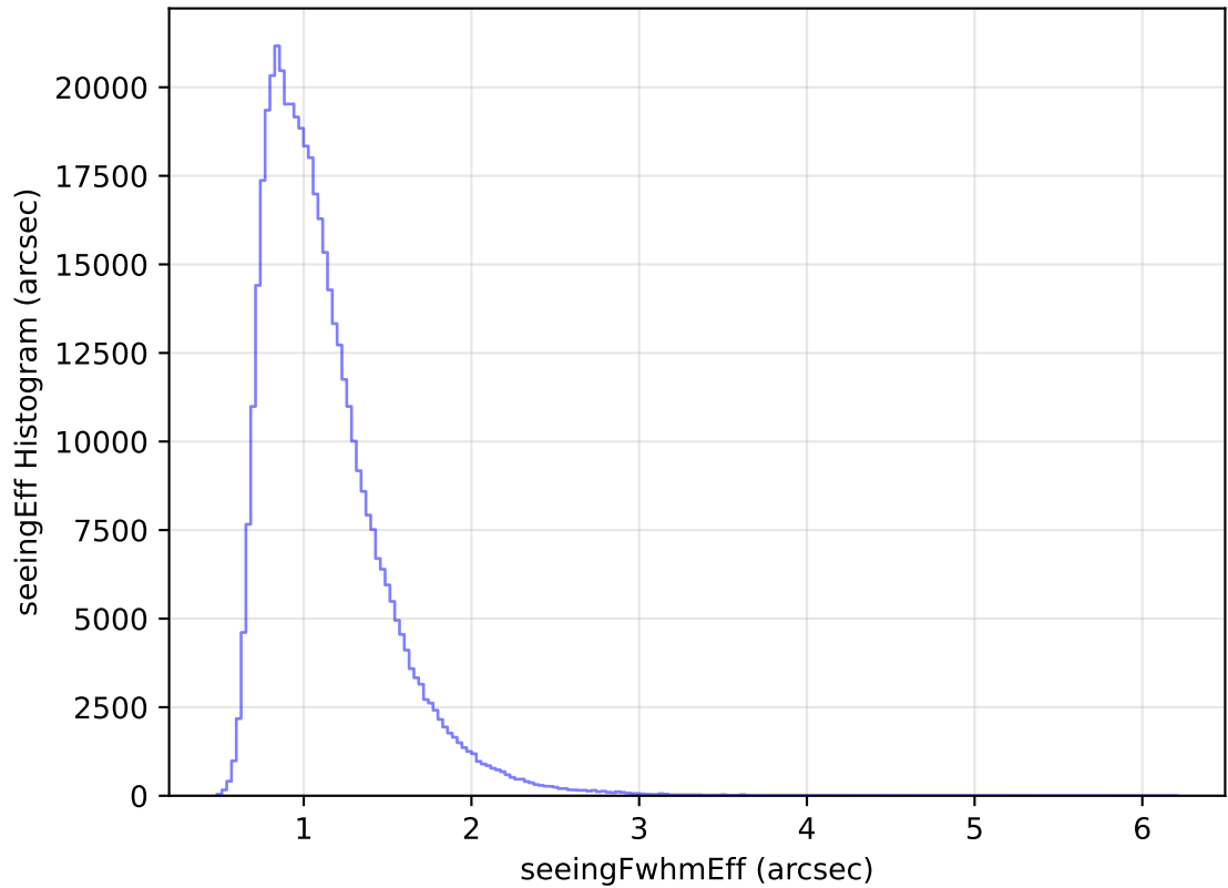
too_elab_heavy_r32_d2_ugrizy_v3.4_10yrs All sky r band: seeingEff Histogram
