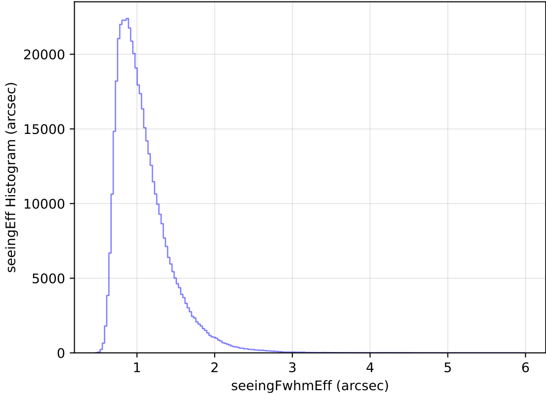
too_elab_heavy_r32_d2_ugrizy_v3.4_10yrs All sky i band: seeingEff Histogram
