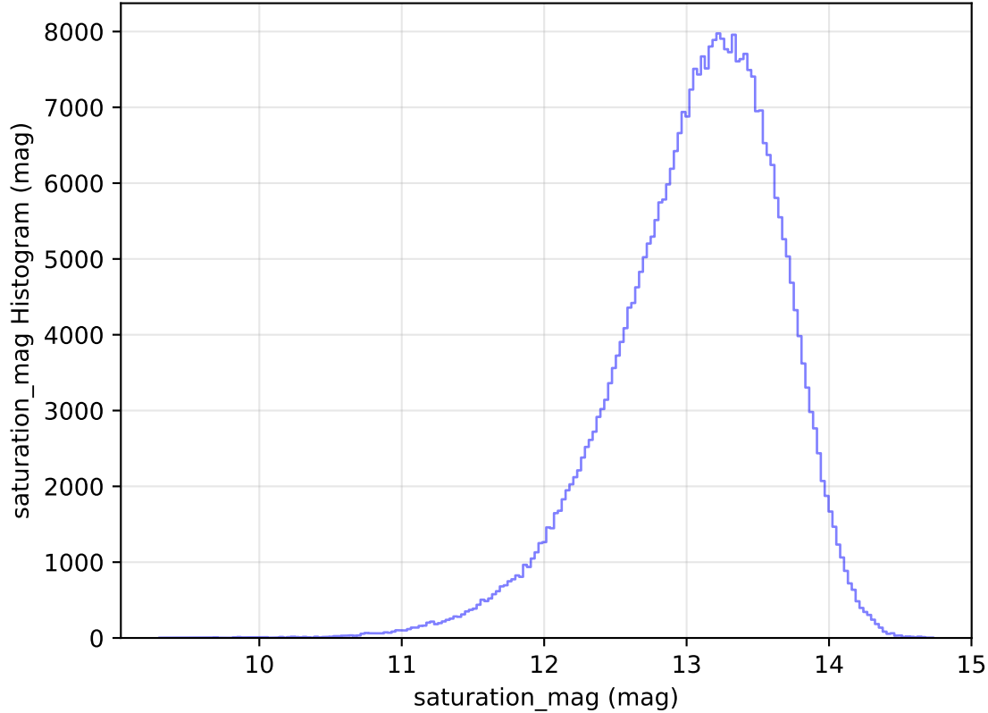
too_elab_heavy_r32_d2_ugrizy_v3.4_10yrs WFD y band: saturation_mag Histogram
