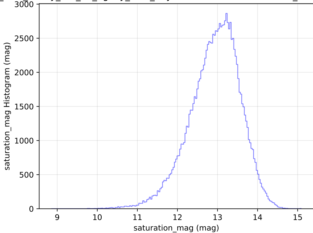
too_elab_heavy_r32_d2_ugrizy_v3.4_10yrs WFD u band: saturation_mag Histogram
