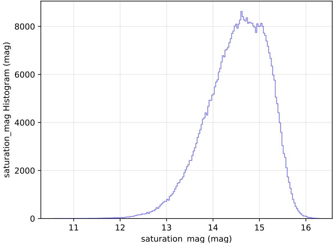
too_elab_heavy_r32_d2_ugrizy_v3.4_10yrs WFD r band: saturation_mag Histogram
