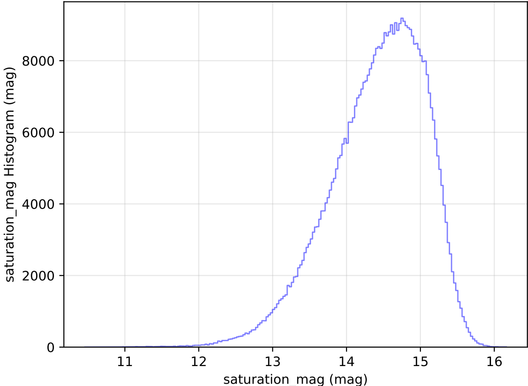
too_elab_heavy_r32_d2_ugrizy_v3.4_10yrs WFD i band: saturation_mag Histogram
