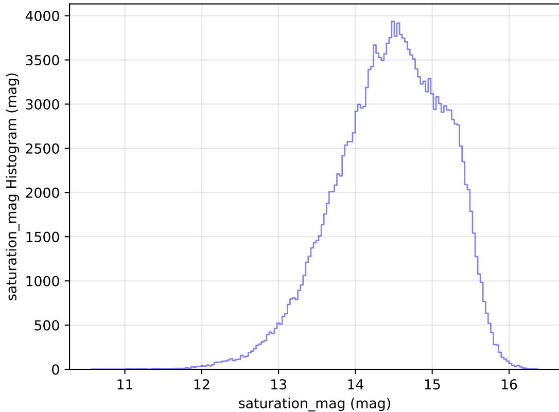
too_elab_heavy_r32_d2_ugrizy_v3.4_10yrs WFD g band: saturation_mag Histogram
