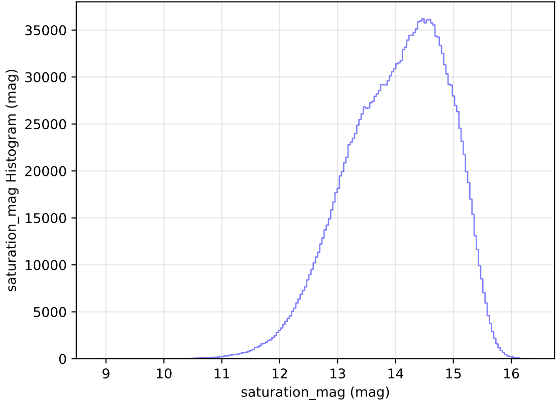
too_elab_heavy_r32_d2_ugrizy_v3.4_10yrs WFD all bands: saturation_mag Histogram
