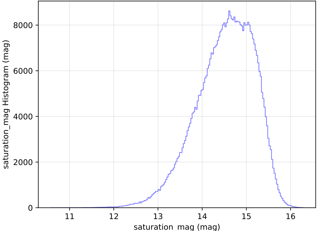
too_elab_heavy_r32_d2_ugrizy_v3.4_10yrs All sky r band: saturation_mag Histogram
