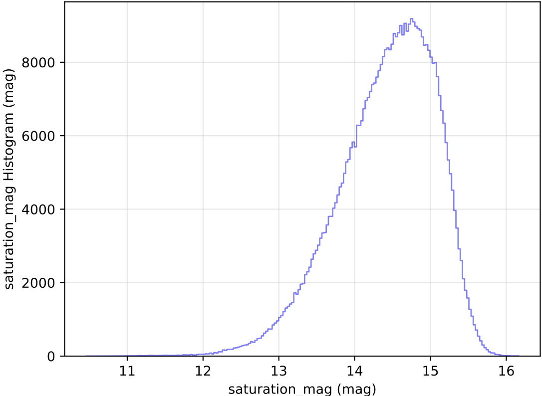
too_elab_heavy_r32_d2_ugrizy_v3.4_10yrs All sky i band: saturation_mag Histogram
