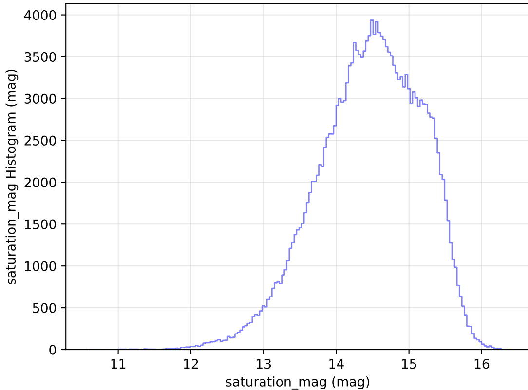
too_elab_heavy_r32_d2_ugrizy_v3.4_10yrs All sky g band: saturation_mag Histogram
