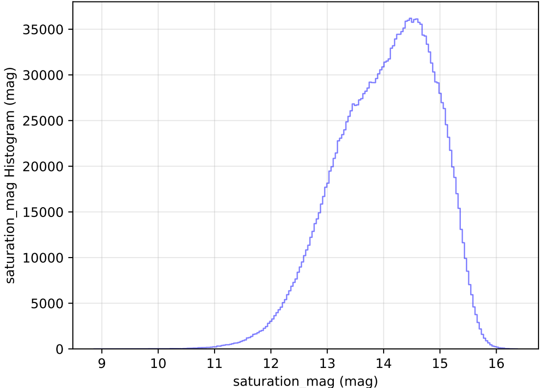
too_elab_heavy_r32_d2_ugrizy_v3.4_10yrs All sky all bands: saturation_mag Histogram
