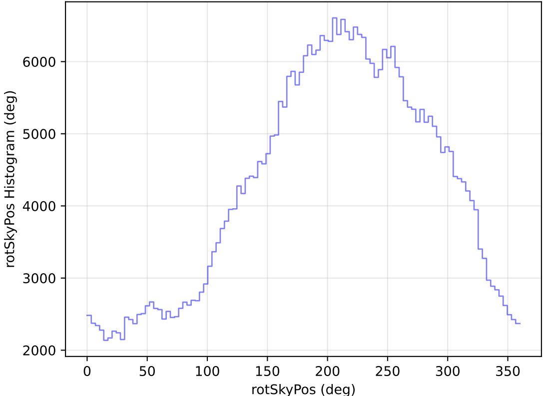
too_elab_heavy_r32_d2_ugrizy_v3.4_10yrs WFD z band: rotSkyPos Histogram
