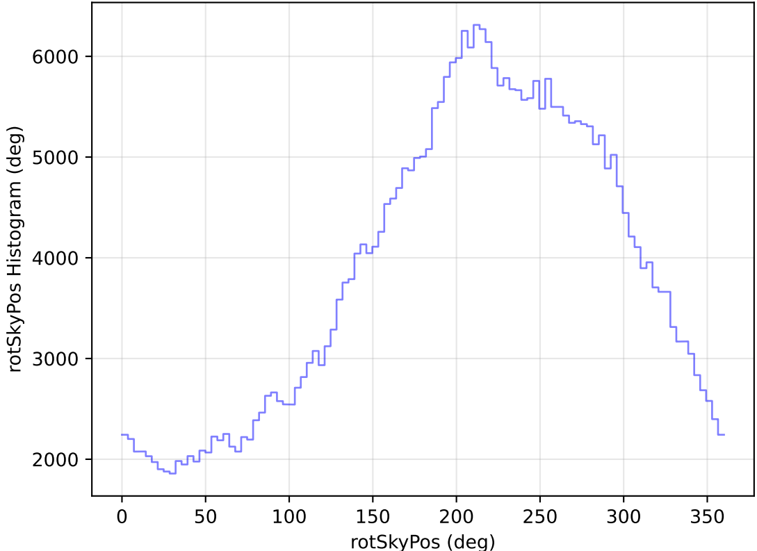
too_elab_heavy_r32_d2_ugrizy_v3.4_10yrs WFD y band: rotSkyPos Histogram
