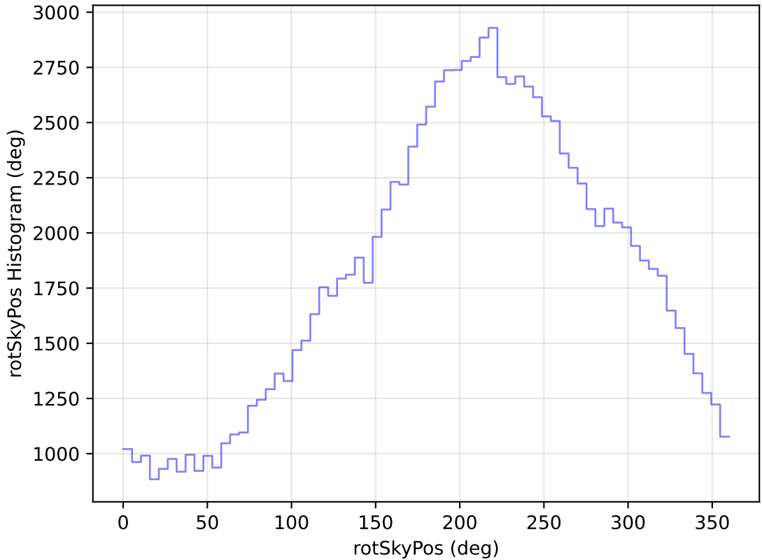
too_elab_heavy_r32_d2_ugrizy_v3.4_10yrs WFD u band: rotSkyPos Histogram
