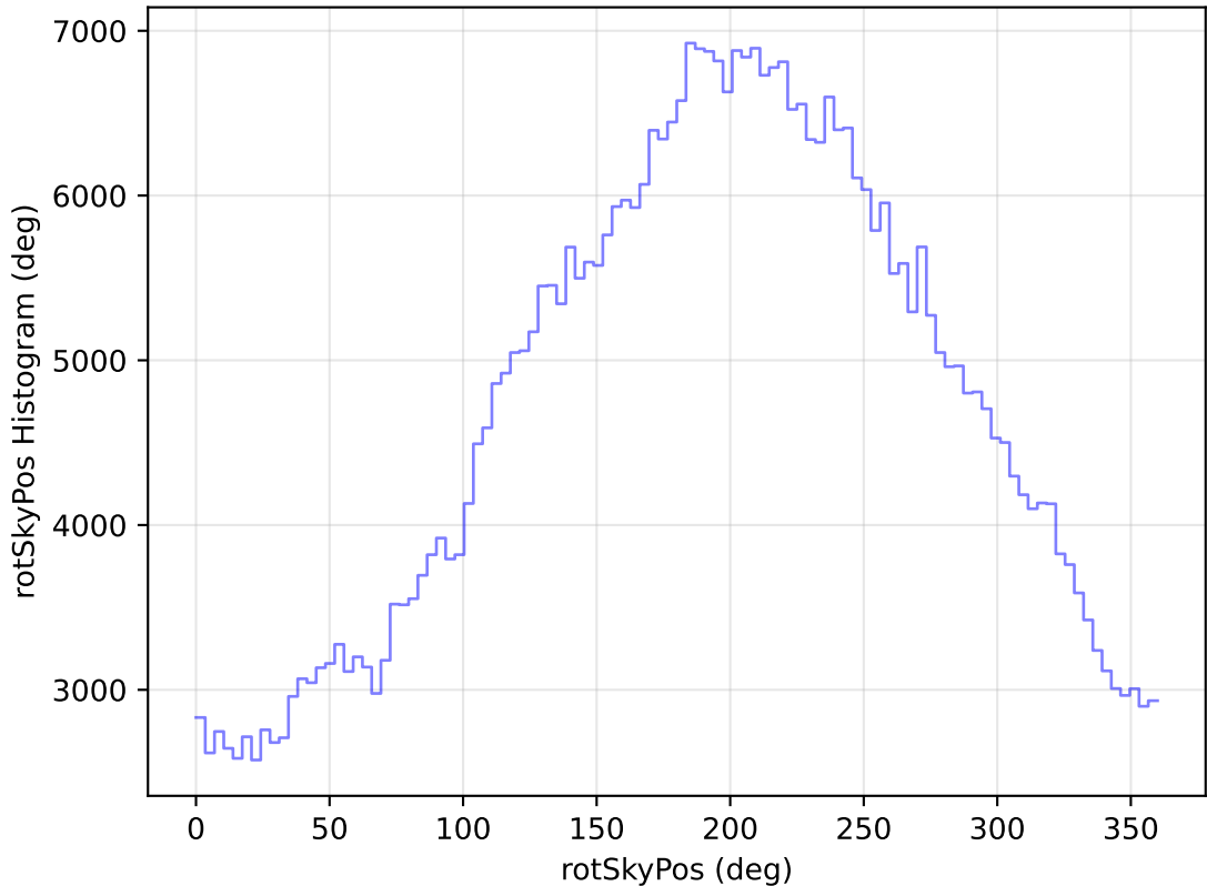
too_elab_heavy_r32_d2_ugrizy_v3.4_10yrs WFD r band: rotSkyPos Histogram
