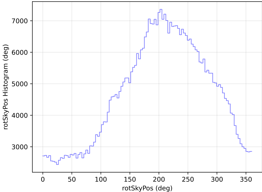
too_elab_heavy_r32_d2_ugrizy_v3.4_10yrs WFD i band: rotSkyPos Histogram
