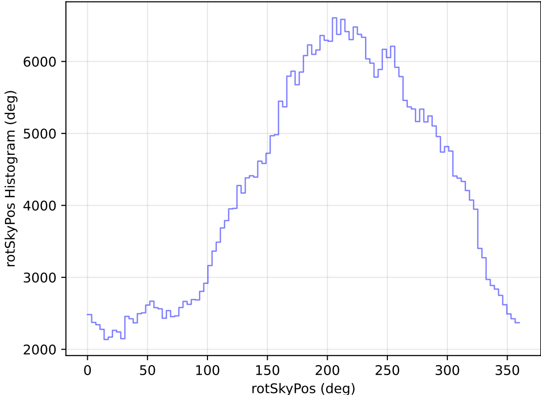
too_elab_heavy_r32_d2_ugrizy_v3.4_10yrs All sky z band: rotSkyPos Histogram
