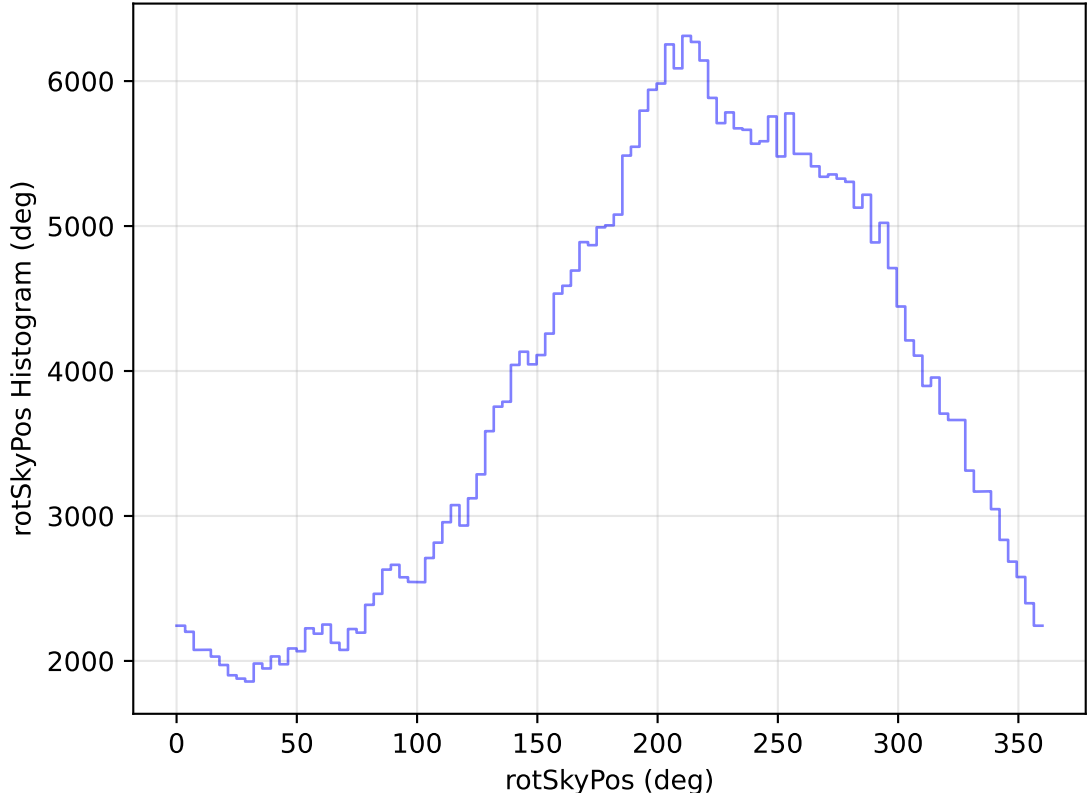
too_elab_heavy_r32_d2_ugrizy_v3.4_10yrs All sky y band: rotSkyPos Histogram
