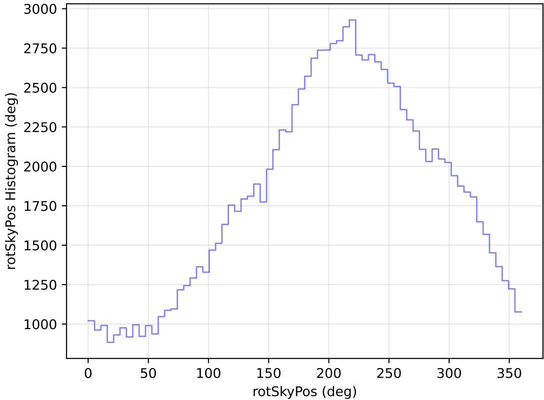
too_elab_heavy_r32_d2_ugrizy_v3.4_10yrs All sky u band: rotSkyPos Histogram
