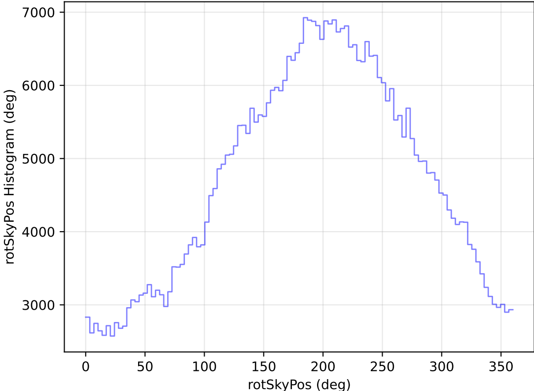
too_elab_heavy_r32_d2_ugrizy_v3.4_10yrs All sky r band: rotSkyPos Histogram
