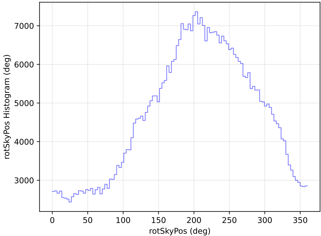
too_elab_heavy_r32_d2_ugrizy_v3.4_10yrs All sky i band: rotSkyPos Histogram
