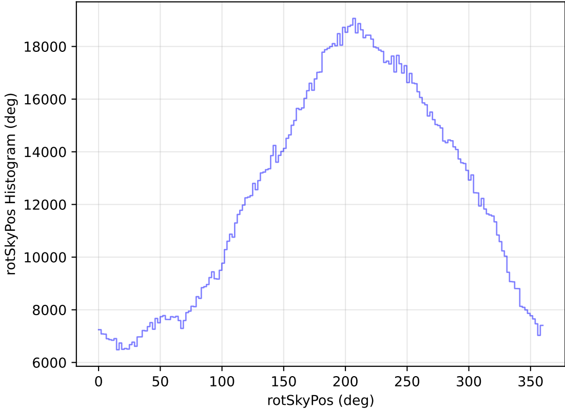
too_elab_heavy_r32_d2_ugrizy_v3.4_10yrs All sky all bands: rotSkyPos Histogram
