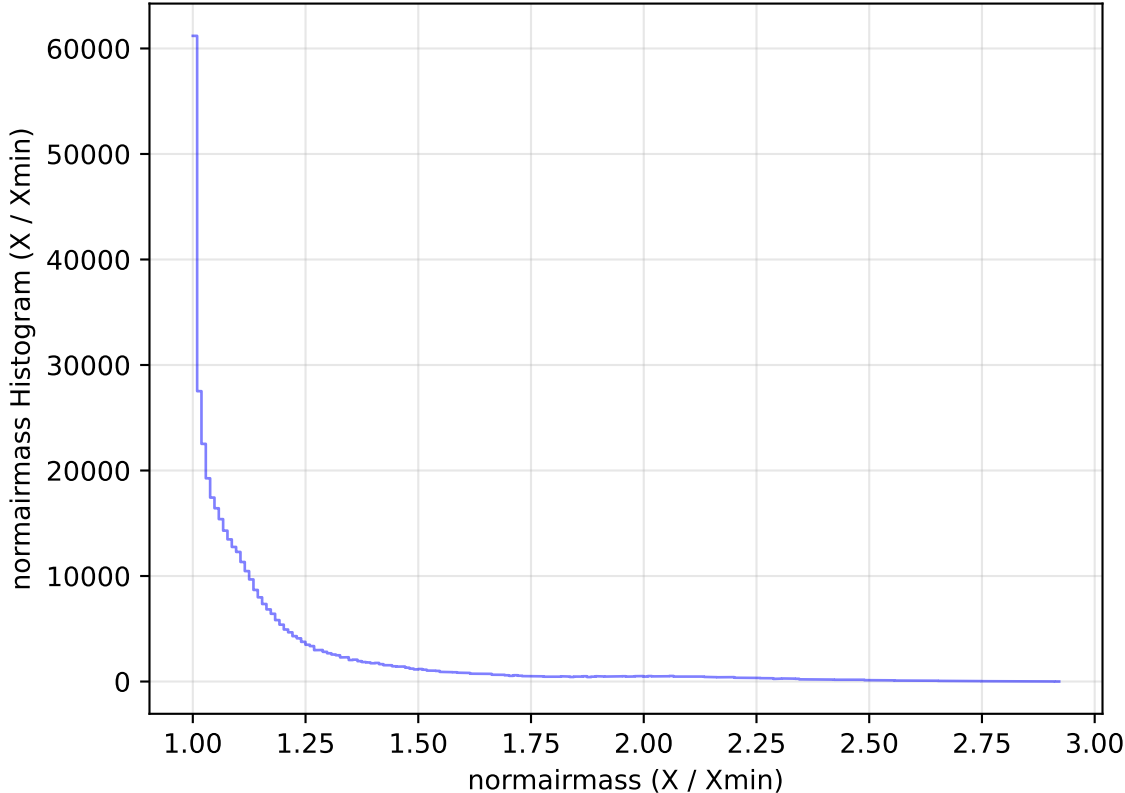
too_elab_heavy_r32_d2_ugrizy_v3.4_10yrs WFD z band: normairmass Histogram
