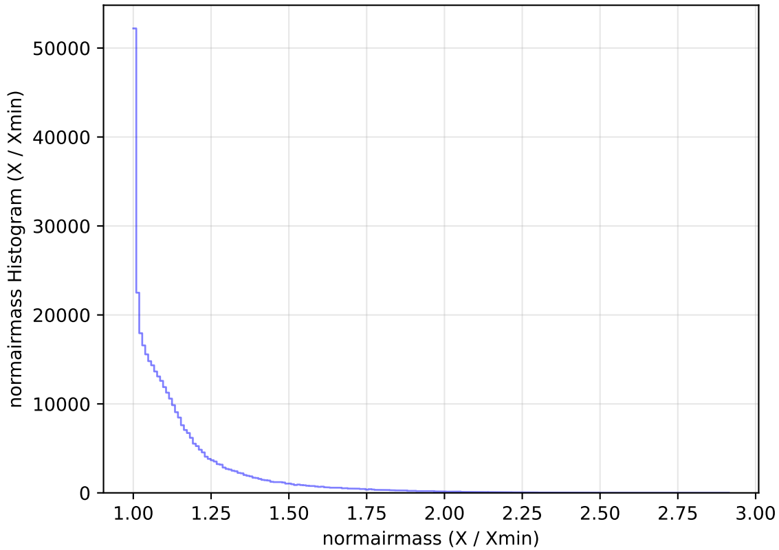
too_elab_heavy_r32_d2_ugrizy_v3.4_10yrs WFD y band: normairmass Histogram
