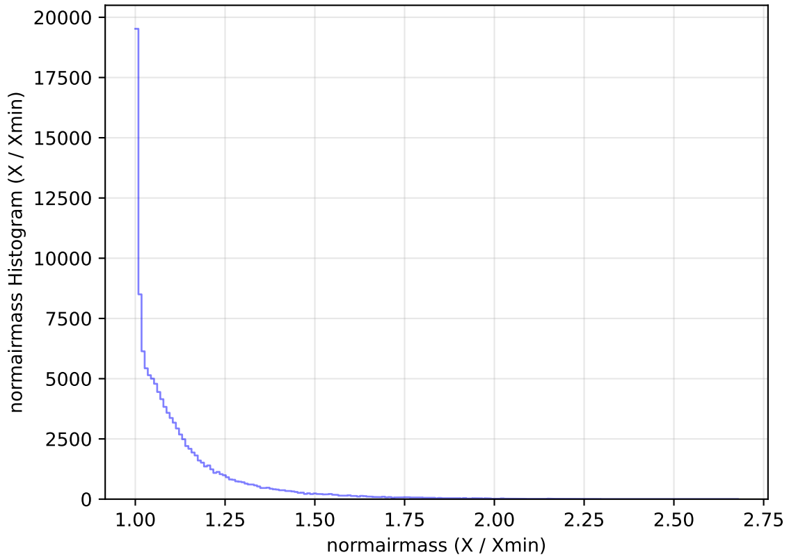
too_elab_heavy_r32_d2_ugrizy_v3.4_10yrs WFD u band: normairmass Histogram
