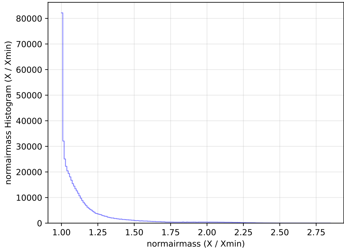
too_elab_heavy_r32_d2_ugrizy_v3.4_10yrs WFD r band: normairmass Histogram
