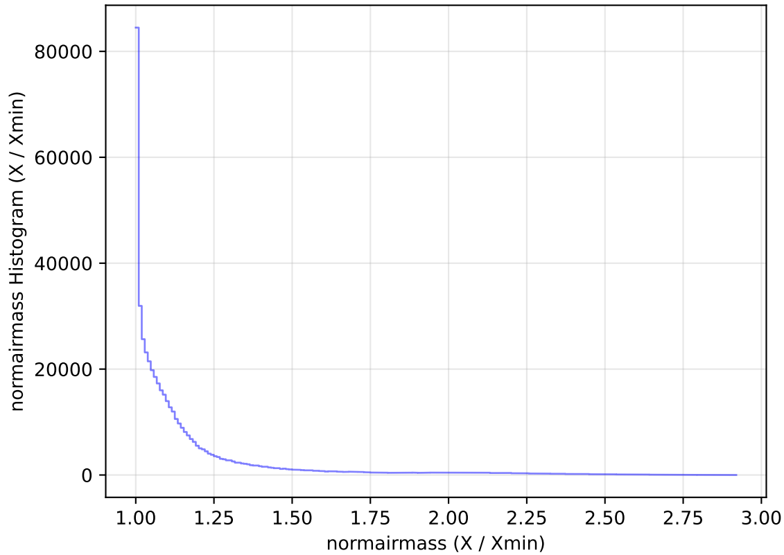
too_elab_heavy_r32_d2_ugrizy_v3.4_10yrs WFD i band: normairmass Histogram
