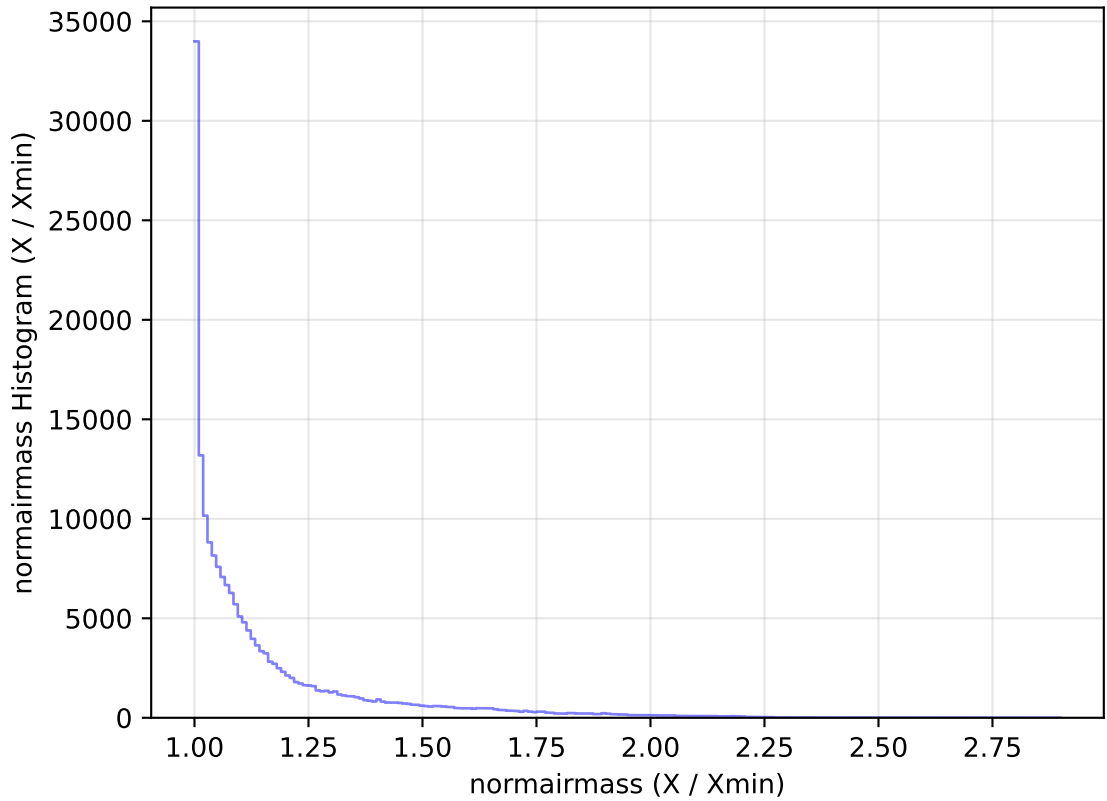
too_elab_heavy_r32_d2_ugrizy_v3.4_10yrs WFD g band: normairmass Histogram
