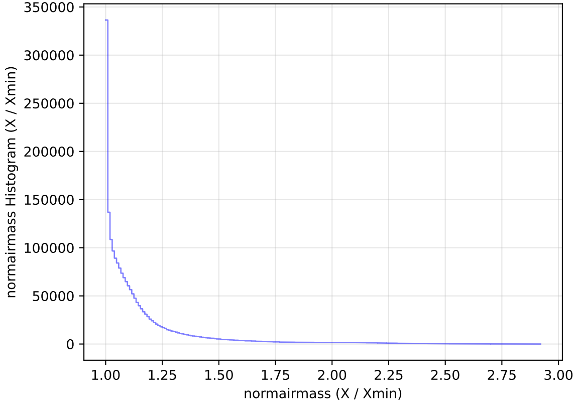
too_elab_heavy_r32_d2_ugrizy_v3.4_10yrs WFD all bands: normairmass Histogram
