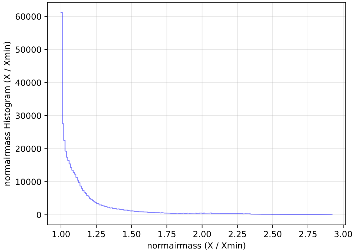
too_elab_heavy_r32_d2_ugrizy_v3.4_10yrs All sky z band: normairmass Histogram
