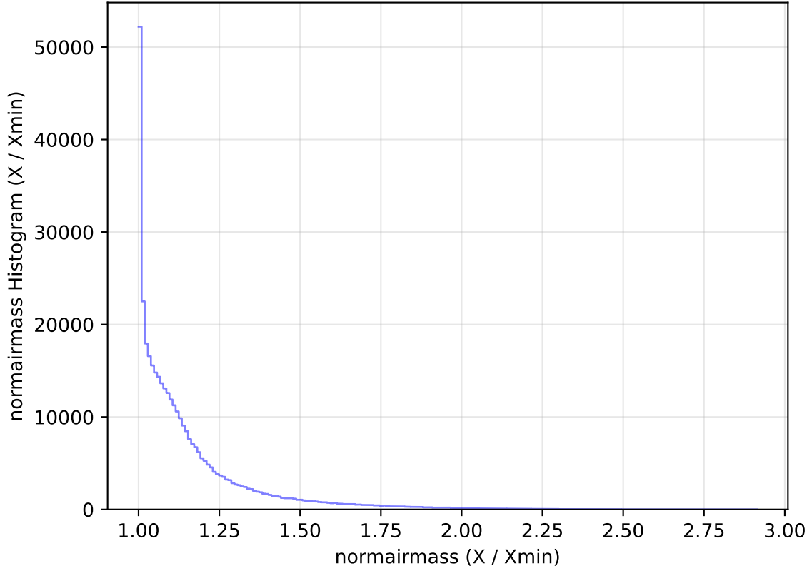
too_elab_heavy_r32_d2_ugrizy_v3.4_10yrs All sky y band: normairmass Histogram
