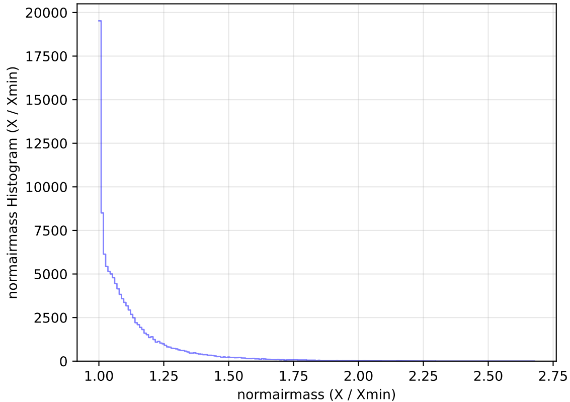
too_elab_heavy_r32_d2_ugrizy_v3.4_10yrs All sky u band: normairmass Histogram
