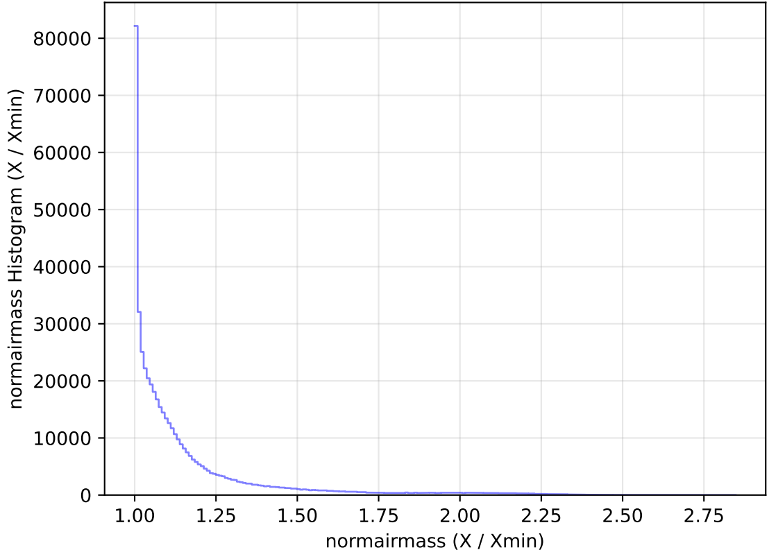
too_elab_heavy_r32_d2_ugrizy_v3.4_10yrs All sky r band: normairmass Histogram
