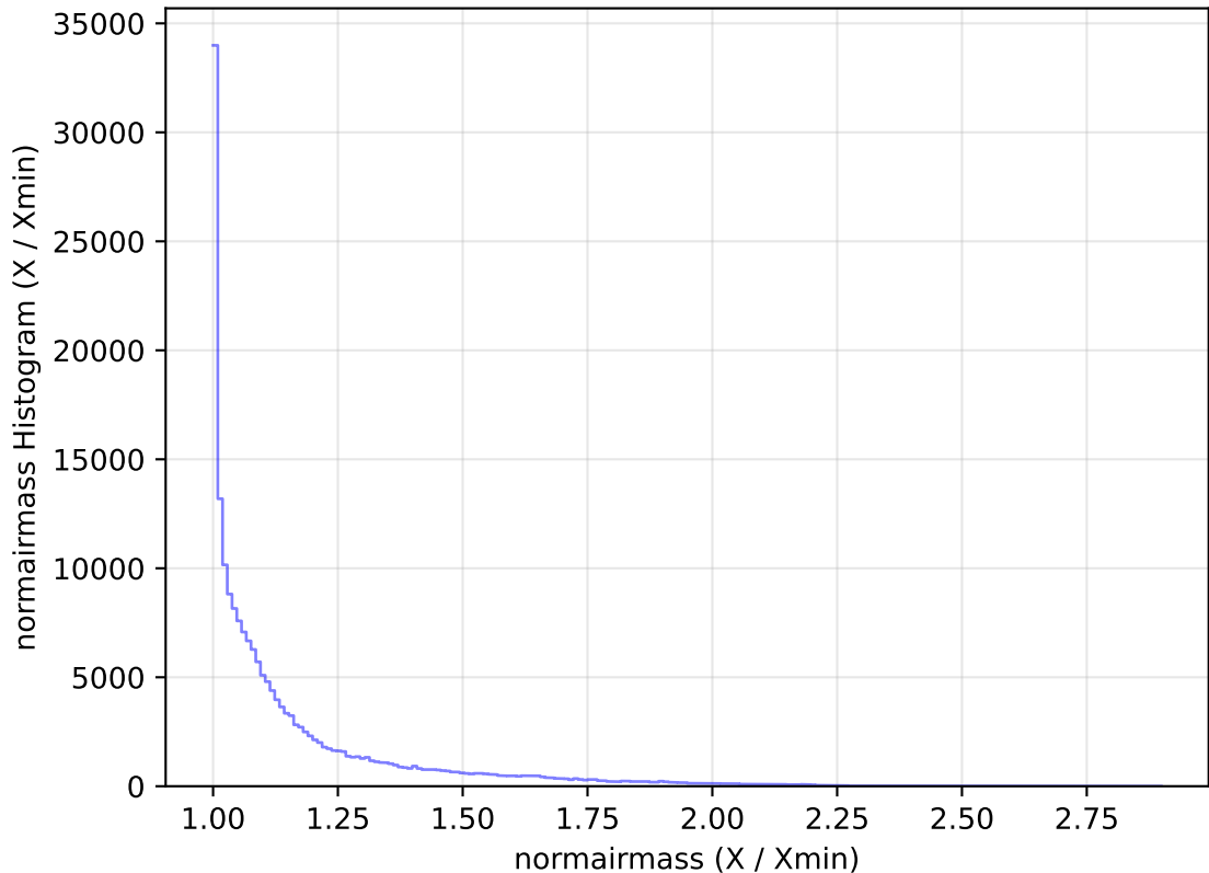
too_elab_heavy_r32_d2_ugrizy_v3.4_10yrs All sky g band: normairmass Histogram
