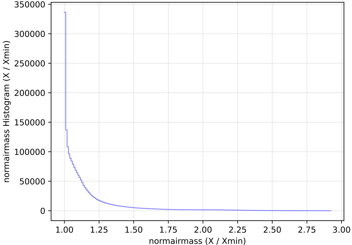
too_elab_heavy_r32_d2_ugrizy_v3.4_10yrs All sky all bands: normairmass Histogram
