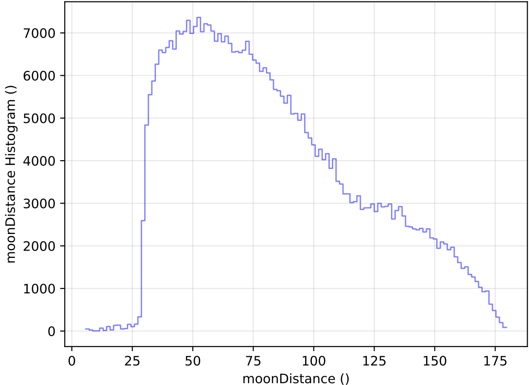
too_elab_heavy_r32_d2_ugrizy_v3.4_10yrs WFD z band: moonDistance Histogram
