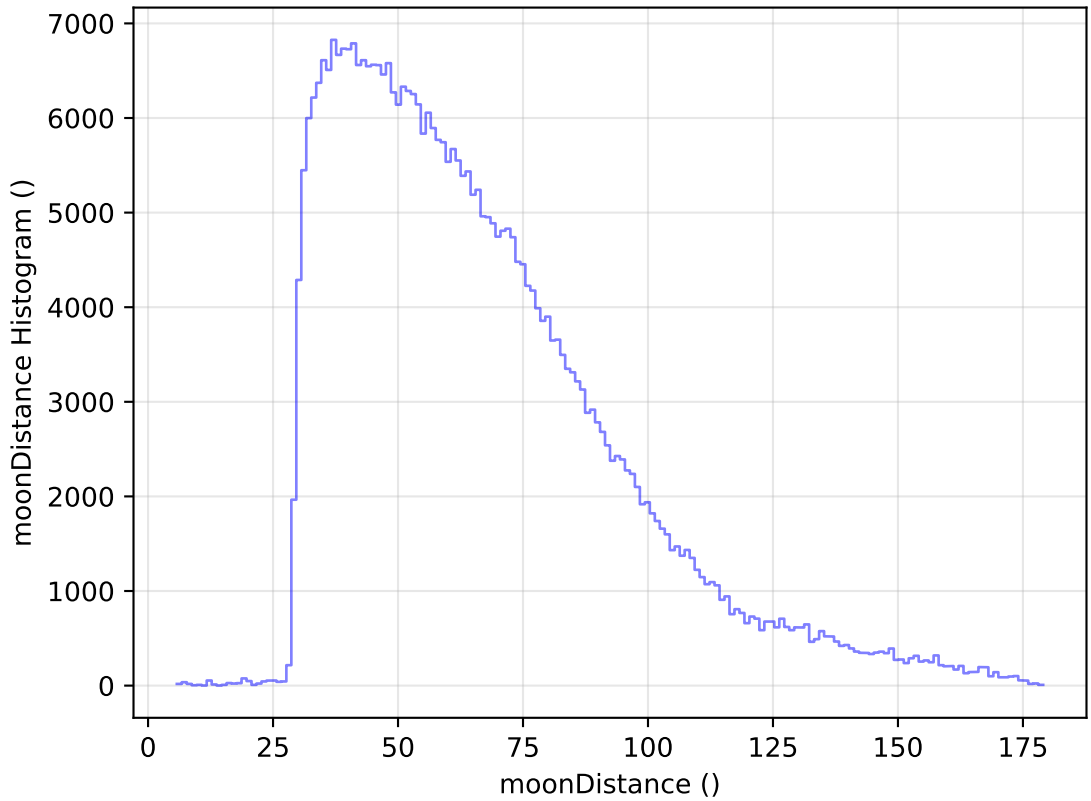
too_elab_heavy_r32_d2_ugrizy_v3.4_10yrs WFD y band: moonDistance Histogram
