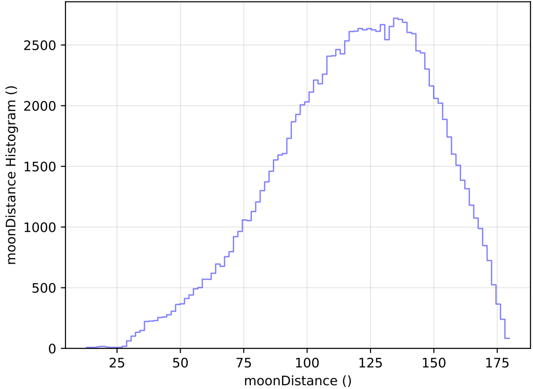
too_elab_heavy_r32_d2_ugrizy_v3.4_10yrs WFD u band: moonDistance Histogram
