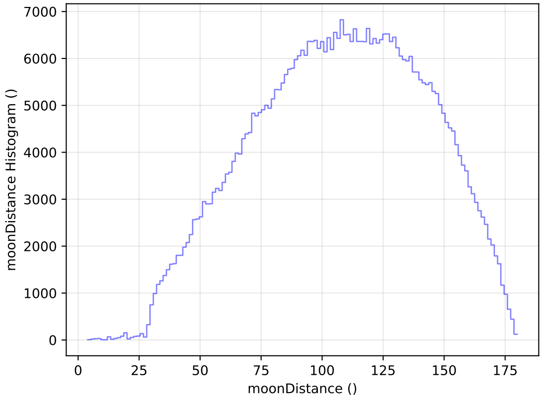
too_elab_heavy_r32_d2_ugrizy_v3.4_10yrs WFD r band: moonDistance Histogram
