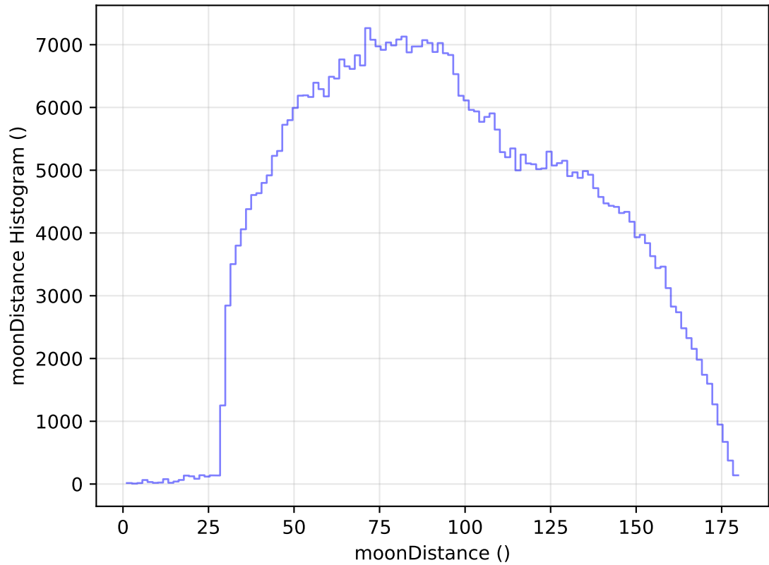
too_elab_heavy_r32_d2_ugrizy_v3.4_10yrs WFD i band: moonDistance Histogram
