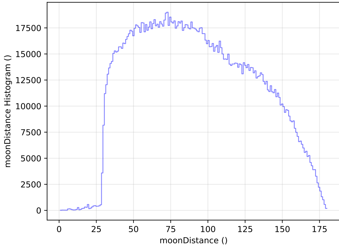
too_elab_heavy_r32_d2_ugrizy_v3.4_10yrs WFD all bands: moonDistance Histogram
