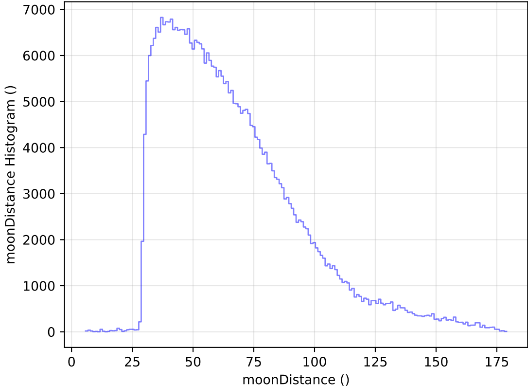
too_elab_heavy_r32_d2_ugrizy_v3.4_10yrs All sky y band: moonDistance Histogram
