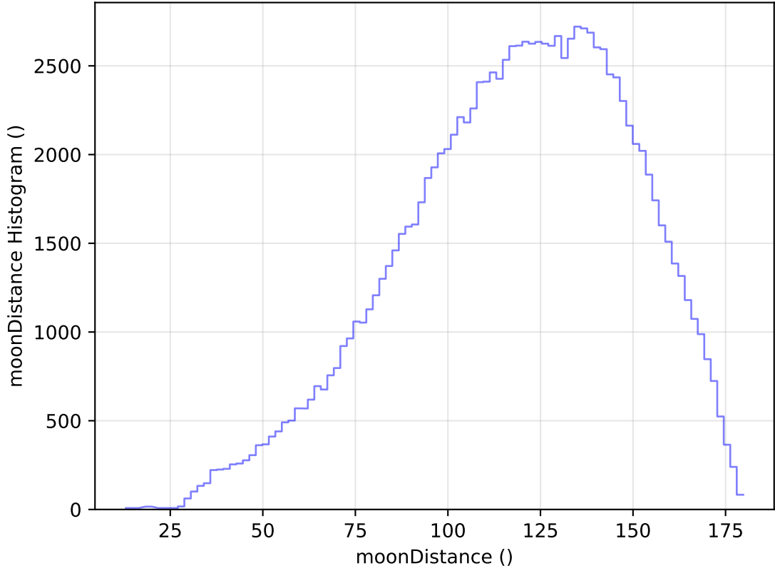
too_elab_heavy_r32_d2_ugrizy_v3.4_10yrs All sky u band: moonDistance Histogram
