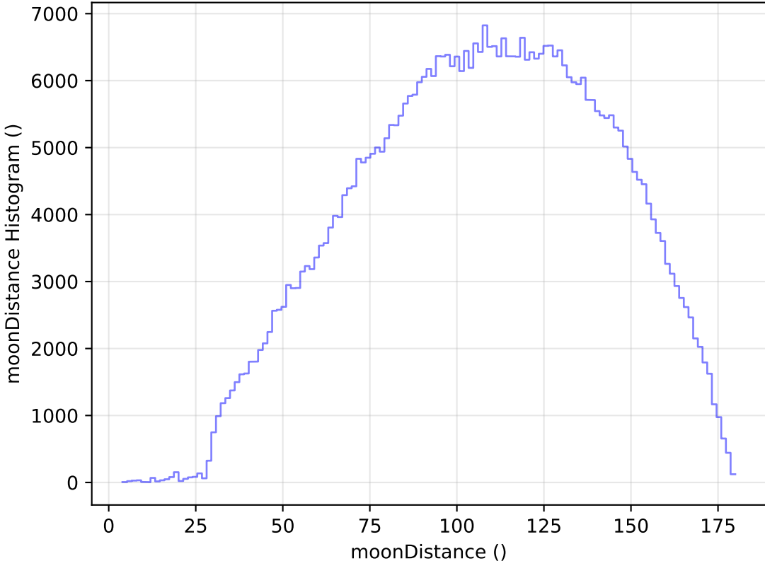
too_elab_heavy_r32_d2_ugrizy_v3.4_10yrs All sky r band: moonDistance Histogram
