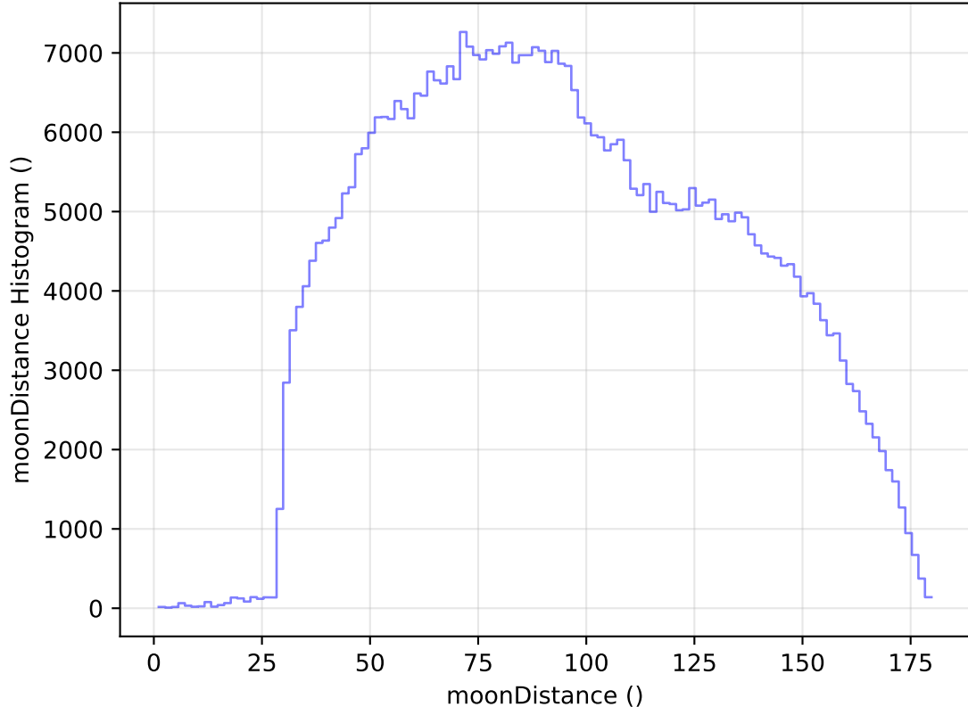
too_elab_heavy_r32_d2_ugrizy_v3.4_10yrs All sky i band: moonDistance Histogram
