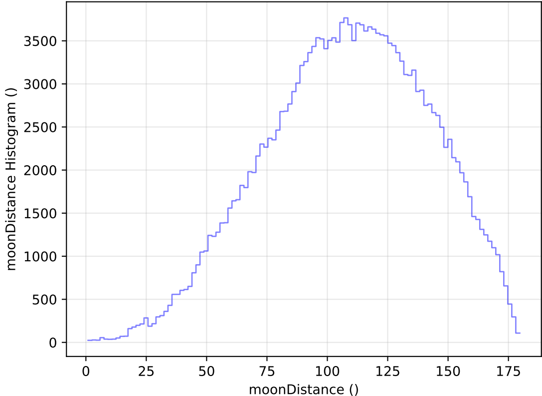
too_elab_heavy_r32_d2_ugrizy_v3.4_10yrs All sky g band: moonDistance Histogram
